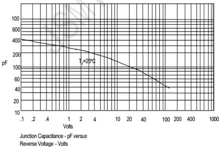
FIG.4-TYPICAL JUNCTION CAPACITANCE
