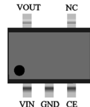
SOT23-5 (Top view)
