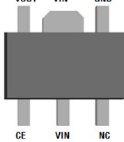
SOT89-5 (Top view)
