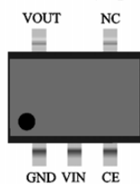
SOT23-5B (Top view)
