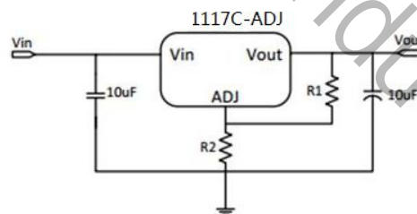
Application Circuit of JSM1117C -ADJ
