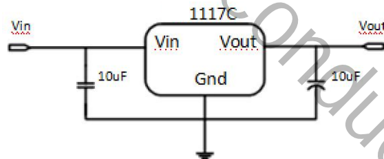
Application circuit of JSM1117C fixed version
