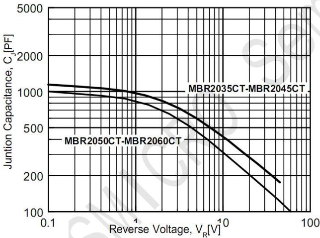
Figure 3. Junction Capacitance
