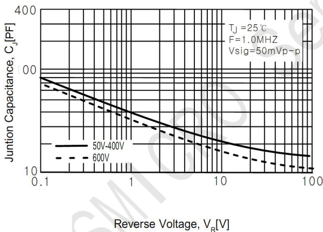
Figure 3. Junction Capacitance
